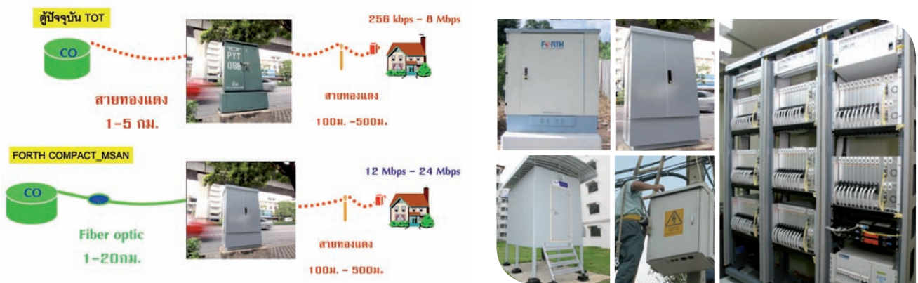
- FORTH Compact-MSAN
